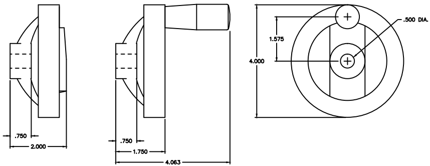
510.11 FOLDING HANDLE ROUND
