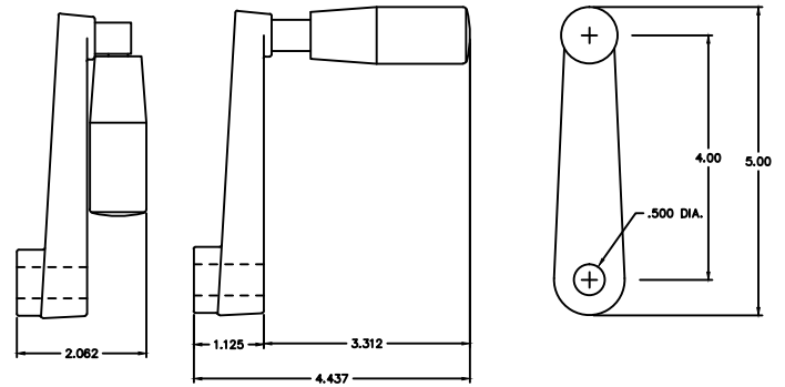
510.12 FOLDING HANDLE STANDARD
